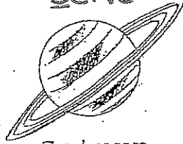
Saturn
